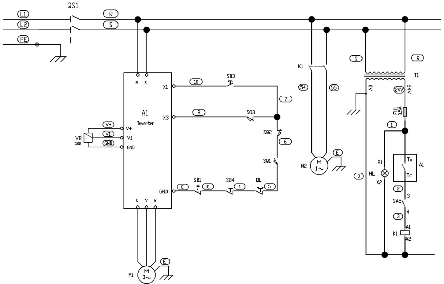
SCHEMA ELECTRIQUE EXPERT 250 SR DAV MONO (VUE 06)
