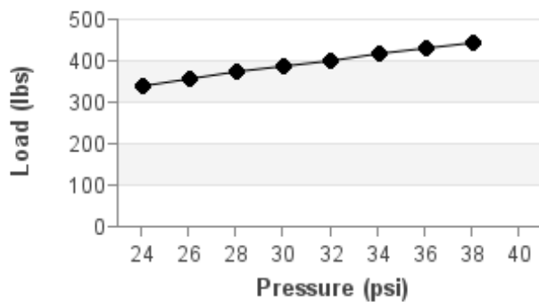
Pressure and Load Adjustments @ Rated Pressure
