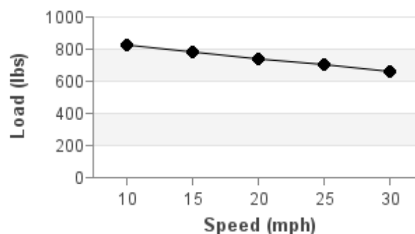
Speed and Load Adjustments @ Rated Pressure
