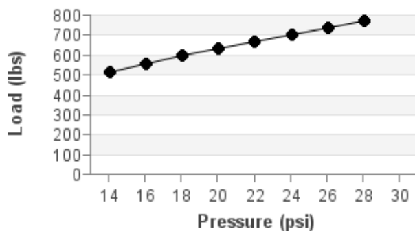
Pressure and Load Adjustments @ Rated Pressure
